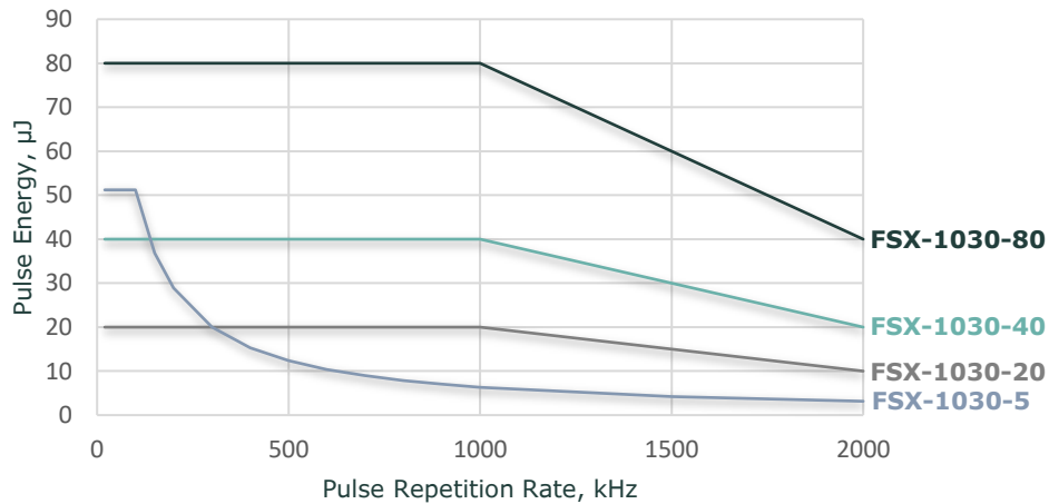
Pulse energy (μJ) as a function of pulse repetition rate (kHz)
